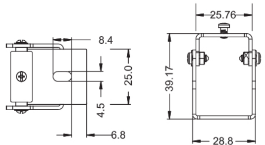
Angle Adjustable Bracket ACC-HX-S2830C2
