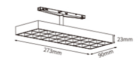
TR11.M13-1 (long-stem for high profile tracks)
