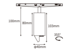
TR11.M6-1 (long-stem for high profile tracks)
