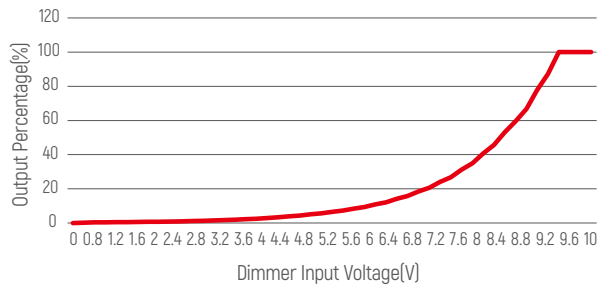
0/1-10V Curve
