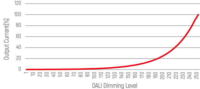
DALI Curve
