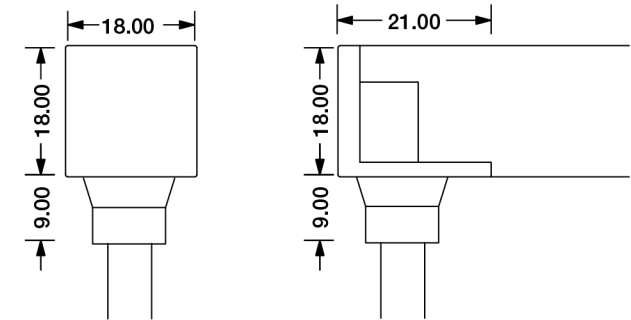
Bottom Entry Connector MJ-SFW20-A-B01/02/03 MJ-SFW20-A-B01SM MJ-SFW20-A-B02SF MJ-SFW20-A-B03SFM
