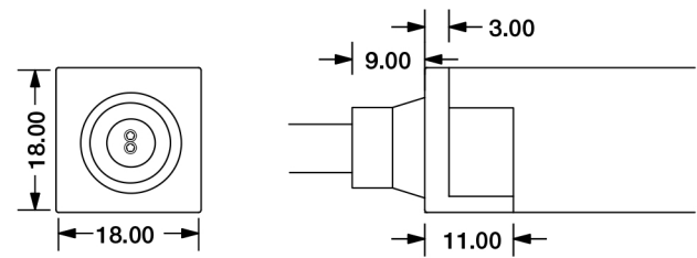
Direct Entry Connector MJ-SFW20-A-D01/02/03 MJ-SFW20-A-D01SM MJ-SFW20-A-D02SF MJ-SFW20-A-D03SFM
