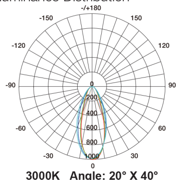
Illuminance Distribution
