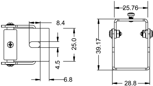
Angle Adjustable Bracket SFW20-ACC-HX-S2830C2
