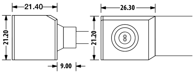
Side Entry Connector MJ-SFW20-A-S01/02/03 MJ-SFW20-A-S01SM MJ-SFW20-A-S02SF MJ-SFW20-A-S03SFM
