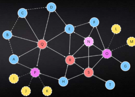
Bluetooth 5.0 SIG Mesh Multi-hop Network Topology
